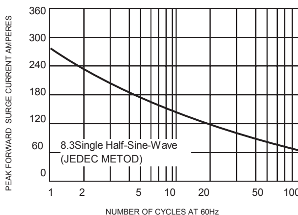
FIG.2-MAXIMUM NON-REPETITIVE SURGE
