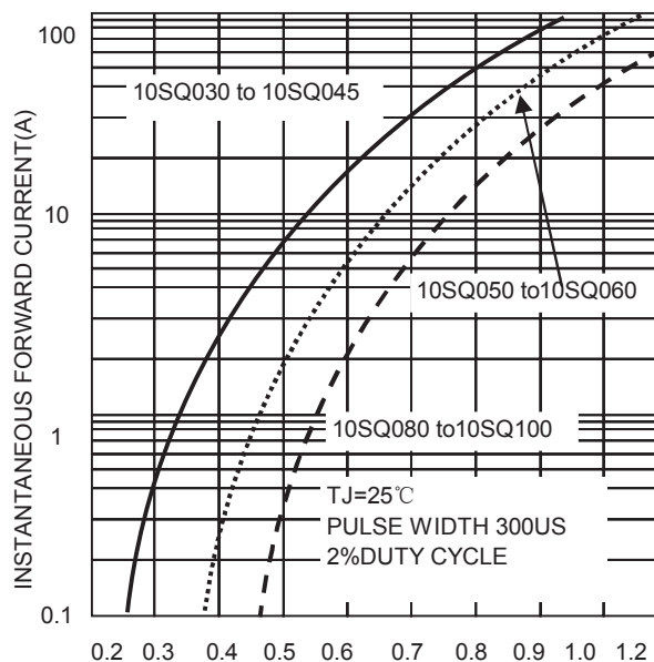
FIG.4-TYPICAL FORWARD CHARACTERISTICS
